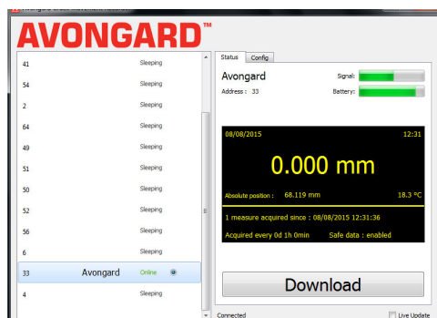
Avongard Crack Movement Recorder Software
